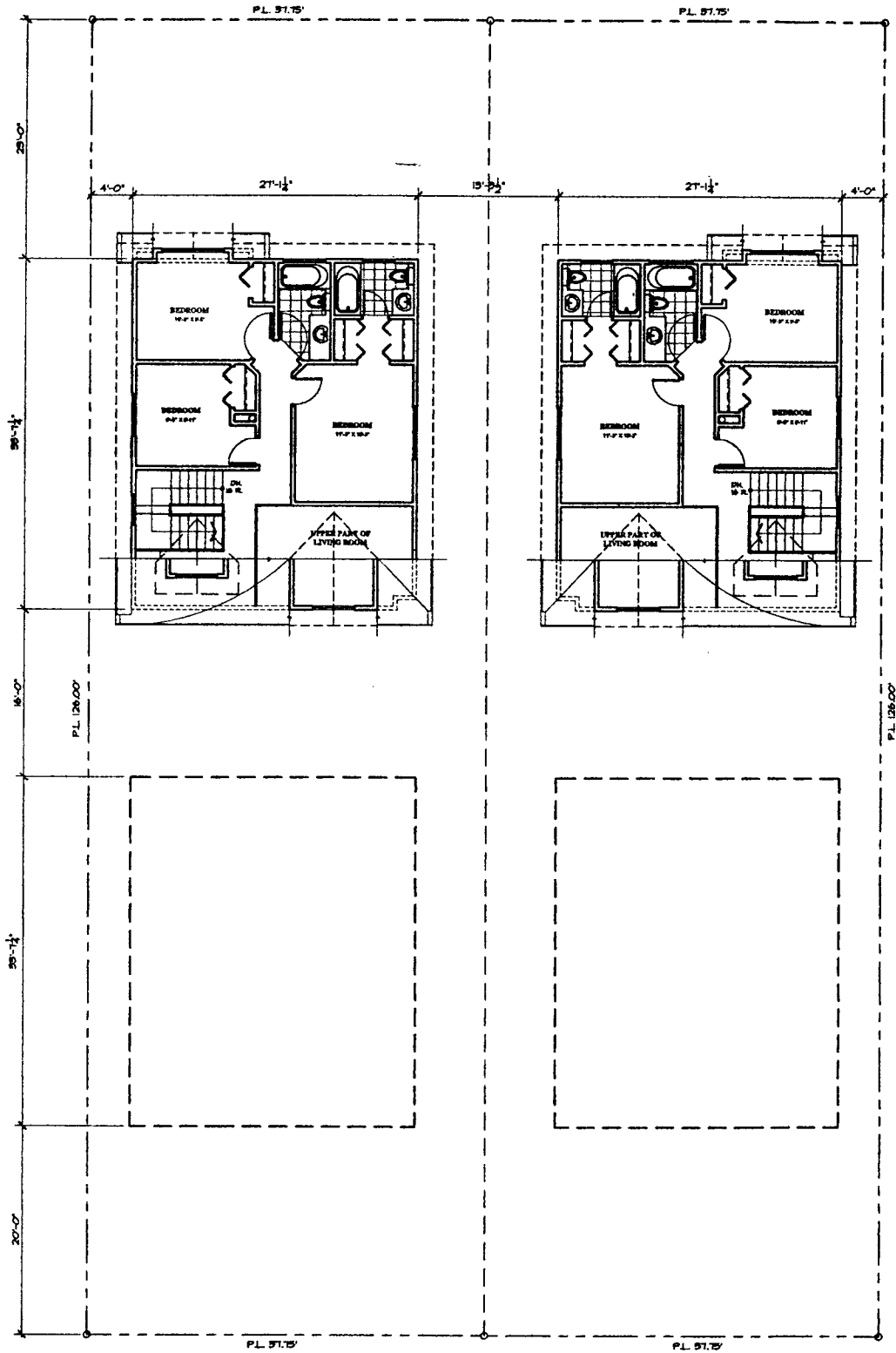
3RD FLOOR PLAN AREA:- REAR UNIT = 759.90 SQ. FT.
