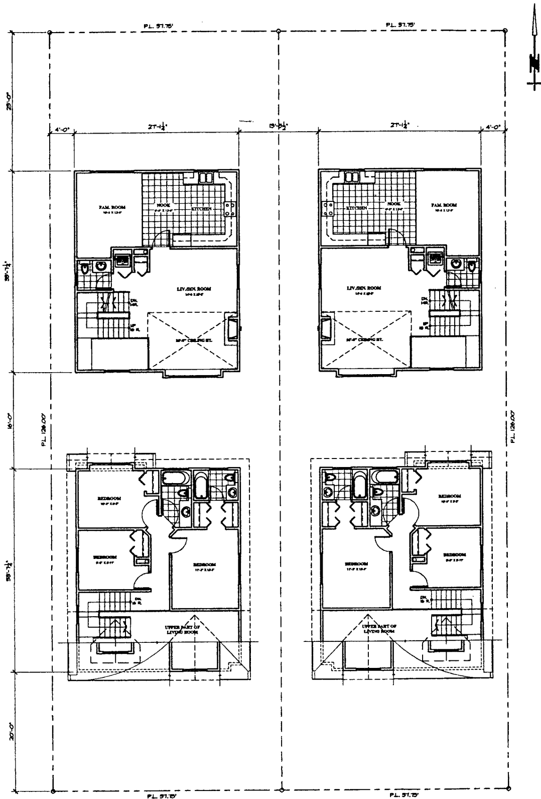
2ND FLOOR PLAN AREA:- FRONT UNIT = 612.44 SQ. FT. REAR UNIT = 856 SQ. FT.
