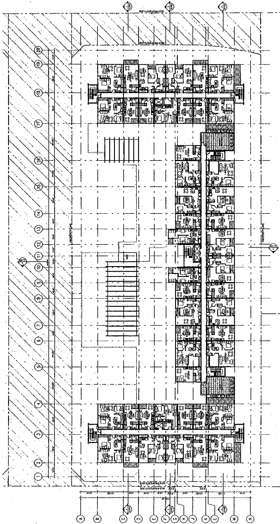
1 LEVEL L3 SCALE 1/8"=1'-0" A204
