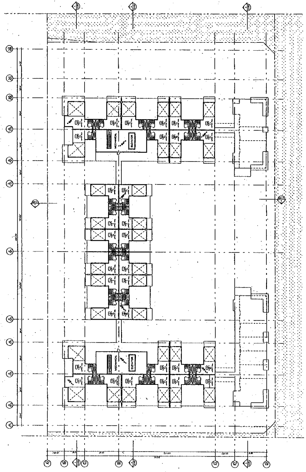
1 LEVEL L4 LOFT PLAN SCALE: 1/8"=1'-0"
