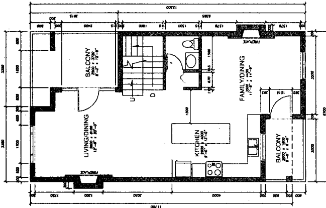
LEVEL 2 SCALE 1:50
