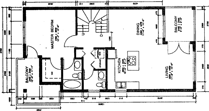
LEVEL 2 a SCALE 1:50
