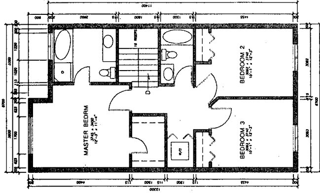
LEVEL 3 SCALE 1:50
