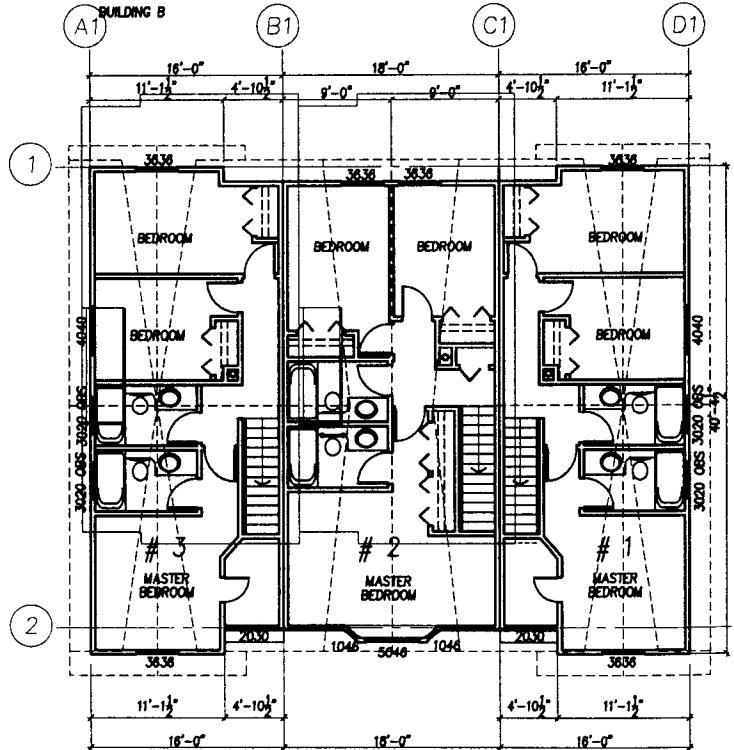
SECOND FLOOR PLAN BUILDING A BUILDING B
