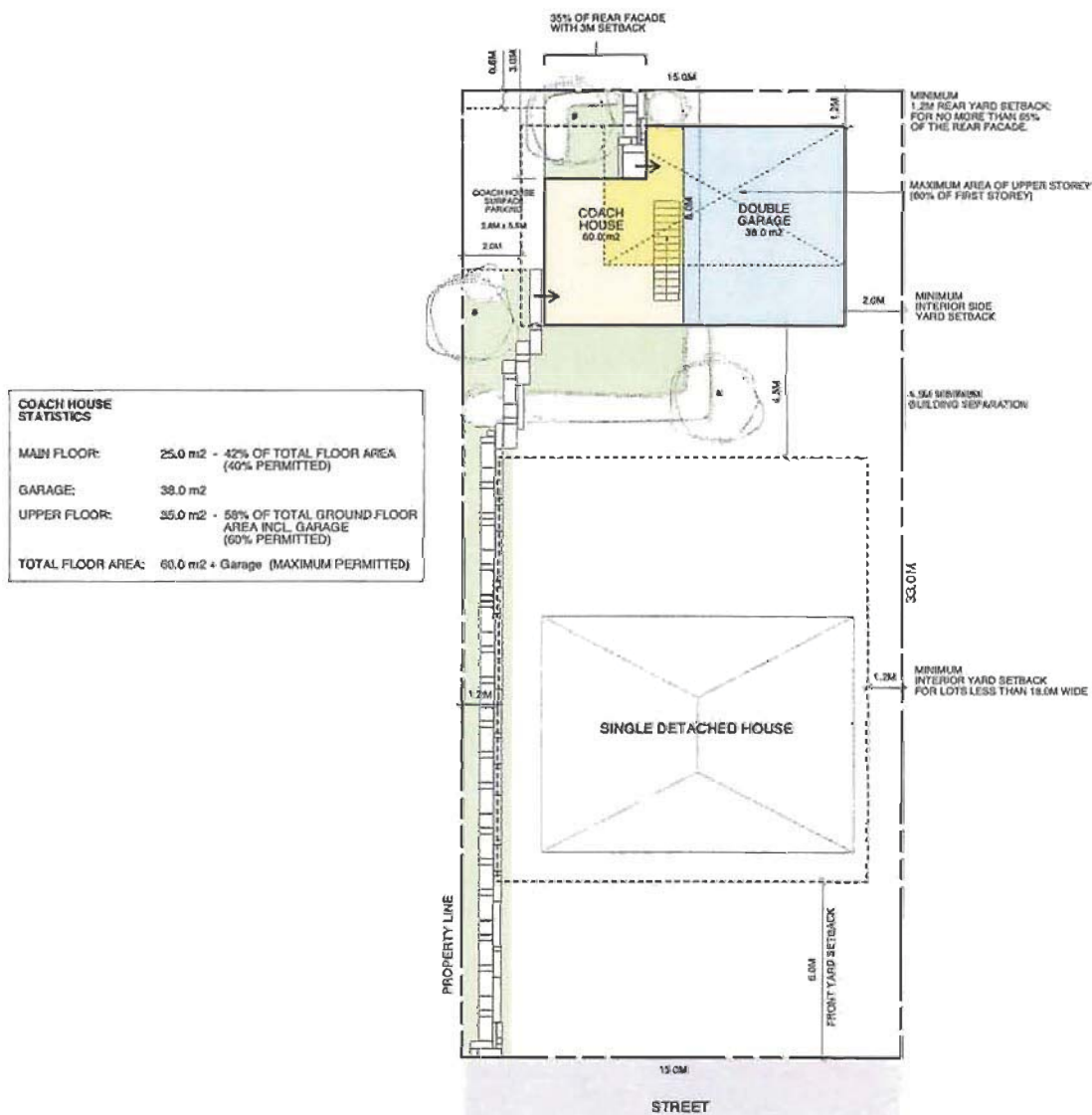
TYPICAL COACH HOUSE SITE PLAN BURKEVILLE, RICHMOND BC SCALE 1:100
