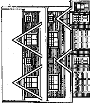
EAST ELEVATION BUILDING B
