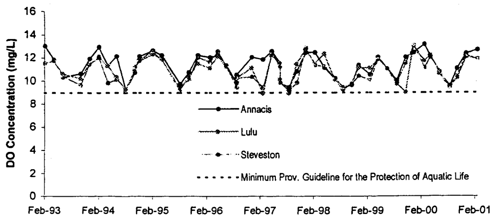
Figure 2d. Downstream Dissolved Oxygen Monitoring, 1993-2001
