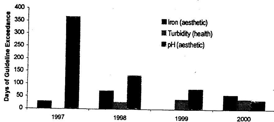
Figure 2g. Seymour Reservoir Drinking Water Quality, 1993-2000
