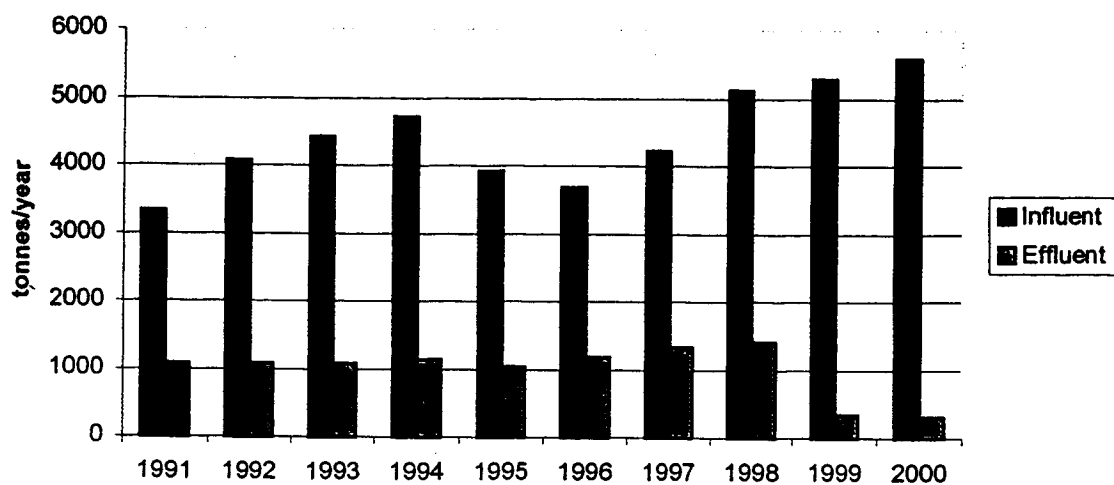
Figure 6l. Lulu Island WTP: Influent vs. Effluent TSS
