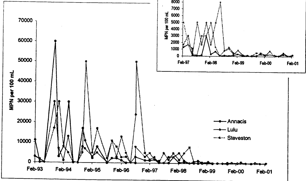
Figure 2a. Downstream Fecal Coliform Monitoring, 1993 - 2001
