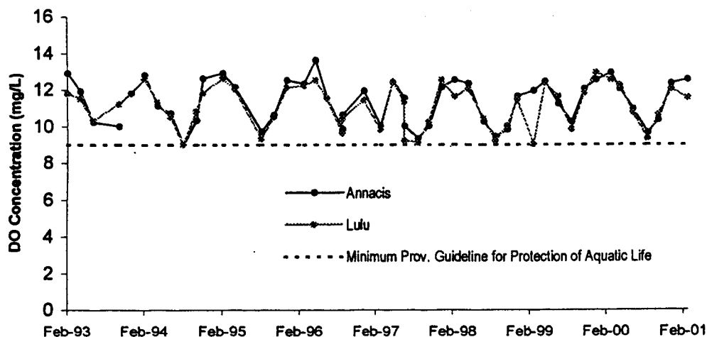
Figure 2c. Upstream Dissolved Oxygen Monitoring, 1993-2001
