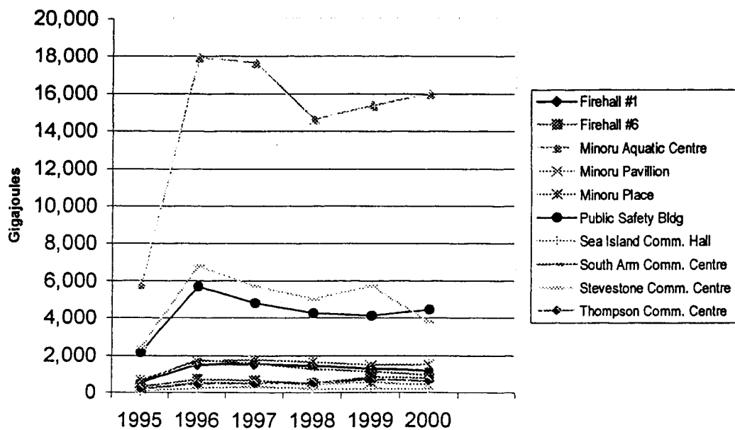
Figure 7b. Natural Gas Consumption (GJ) for Selected City-operated Facilities
