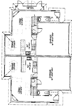
UNIT A1 BUILDING NO. 9 GROUND FLOOR PLAN SCALE 1/8" = 1'-0"
