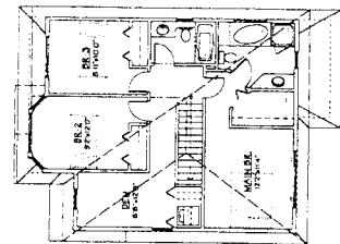
UNIT A2 BUILDING NO. 2, 4, 6 & 10 SECOND FLOOR PLAN SCALE 1/8" = 1'-0"
