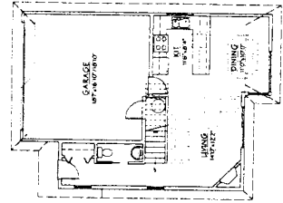
UNIT A1 BUILDING NO. 2, 4, 6 & 10 GROUND FLOOR PLAN SCALE 1/8" = 1'-0"
