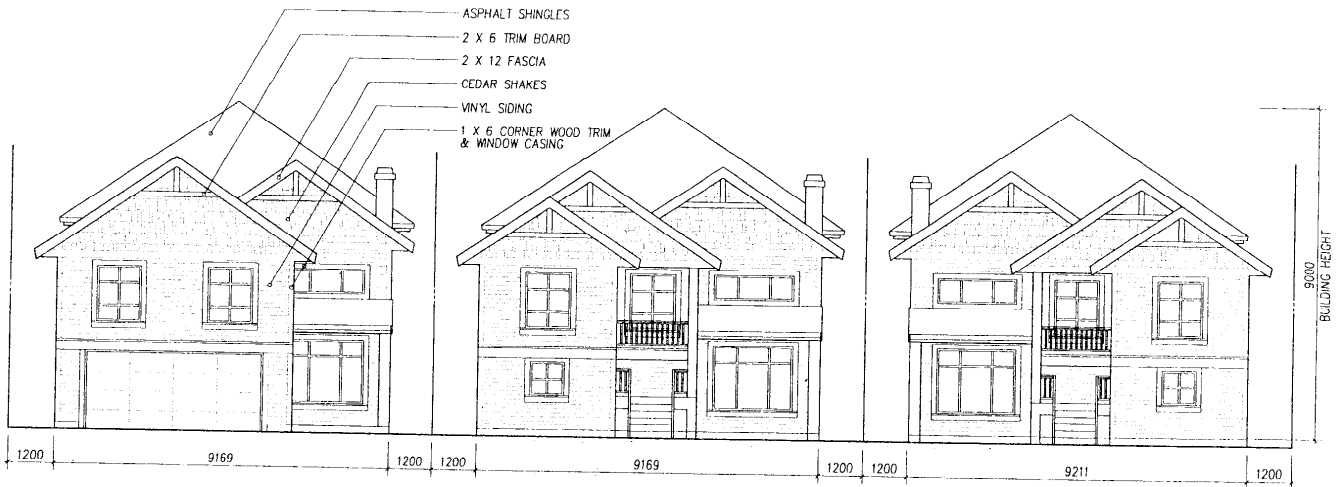
NORTH ELEVATION (WILLIAMS ROAD)
